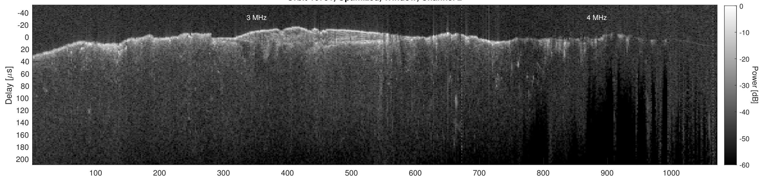
Orbit 10751, Cluttergram
