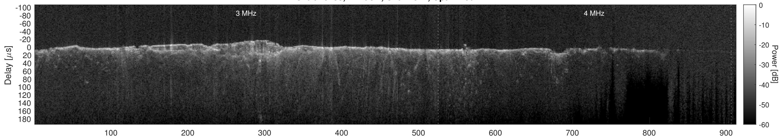
Orbit 10753, Cluttergram
