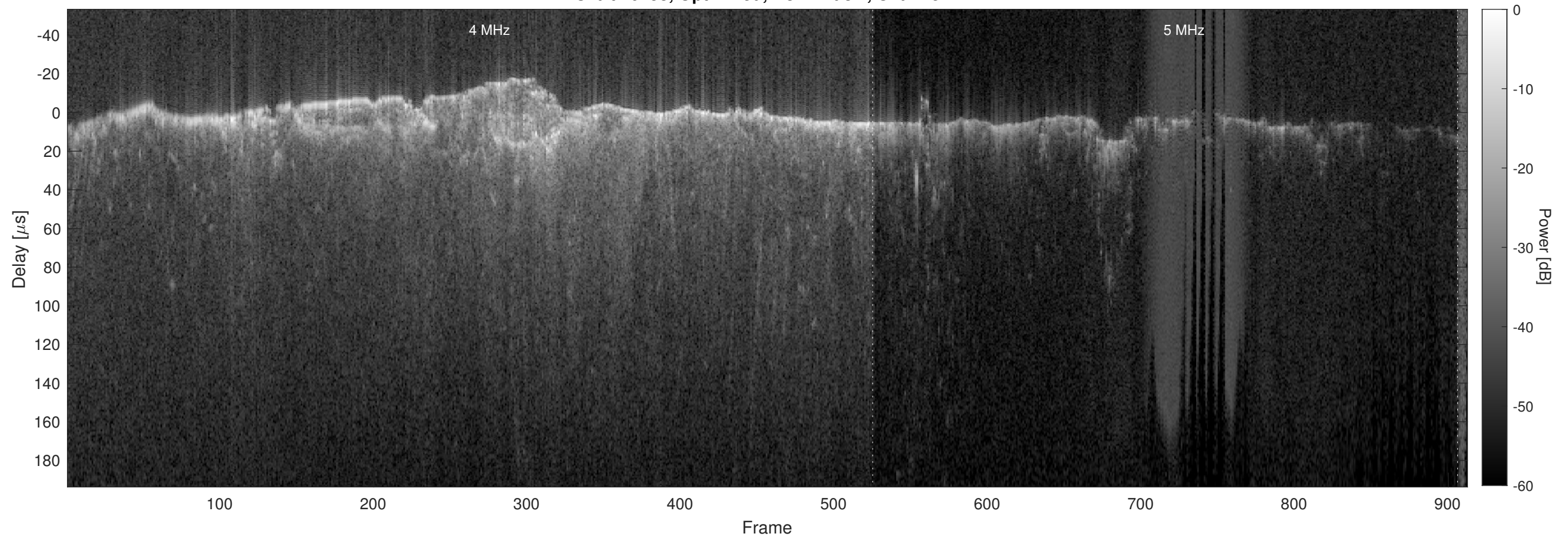
Orbit 10753, Optimized, No Window, Channel 2
