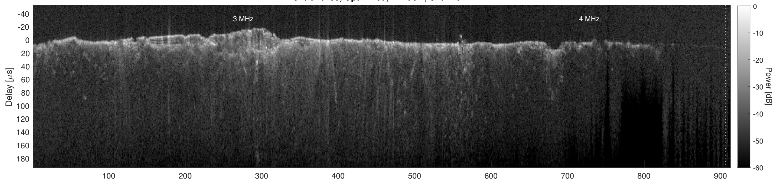
Orbit 10753, Cluttergram
