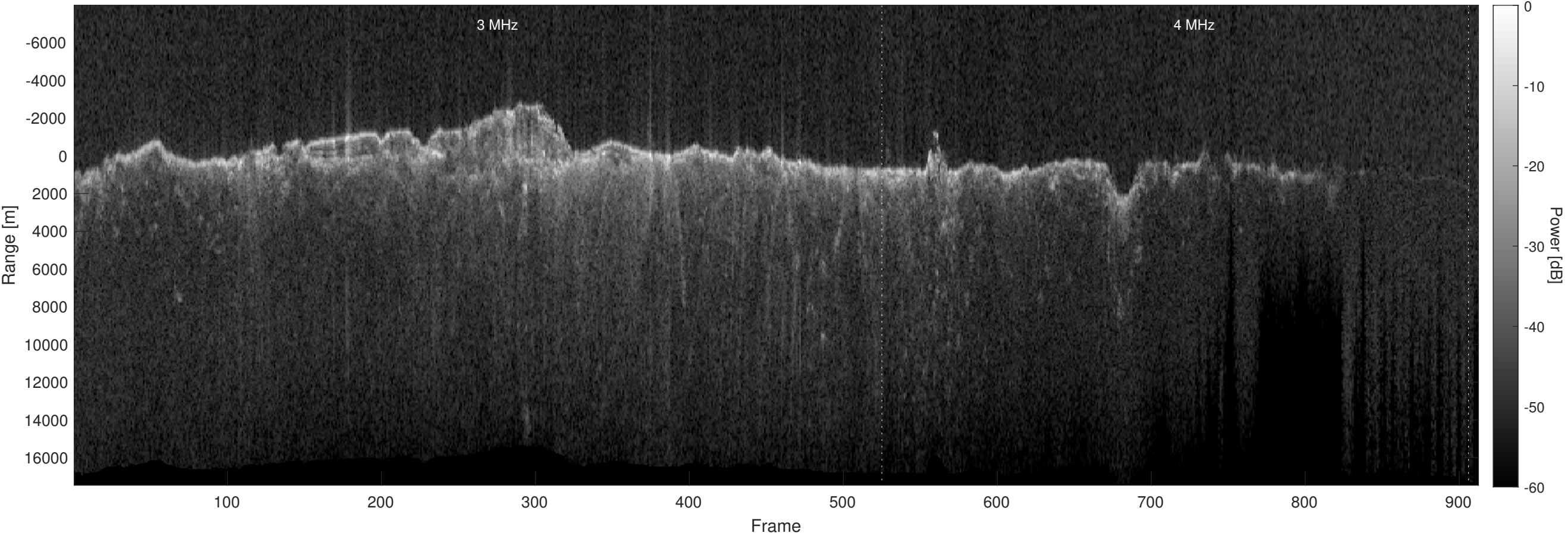
Orbit 10753, Optimized, Window, Depth-Corrected, Channel 2
