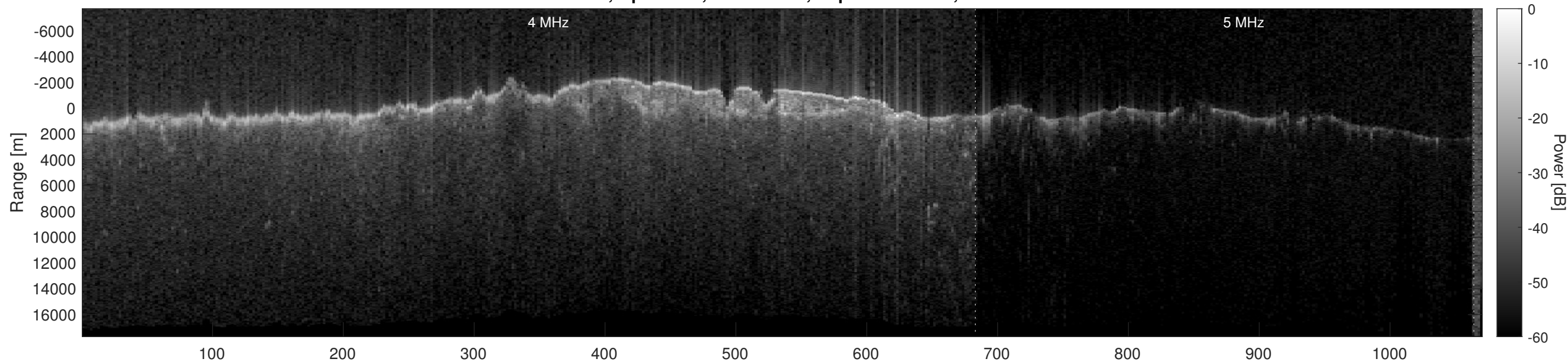
Orbit 10755, Optimized, No Window, Depth-Corrected, Channel 2
