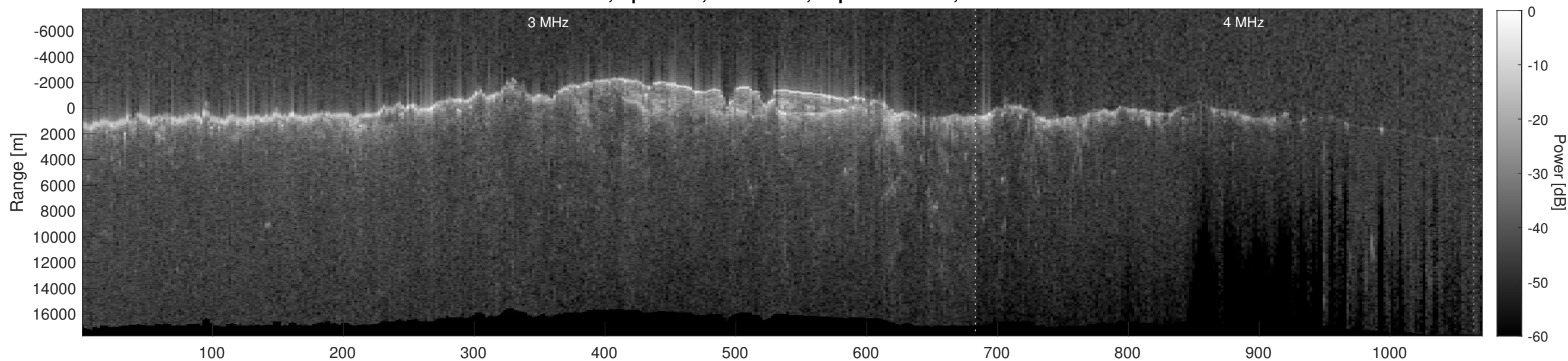
Orbit 10755, Depth-Corrected Cluttergram
