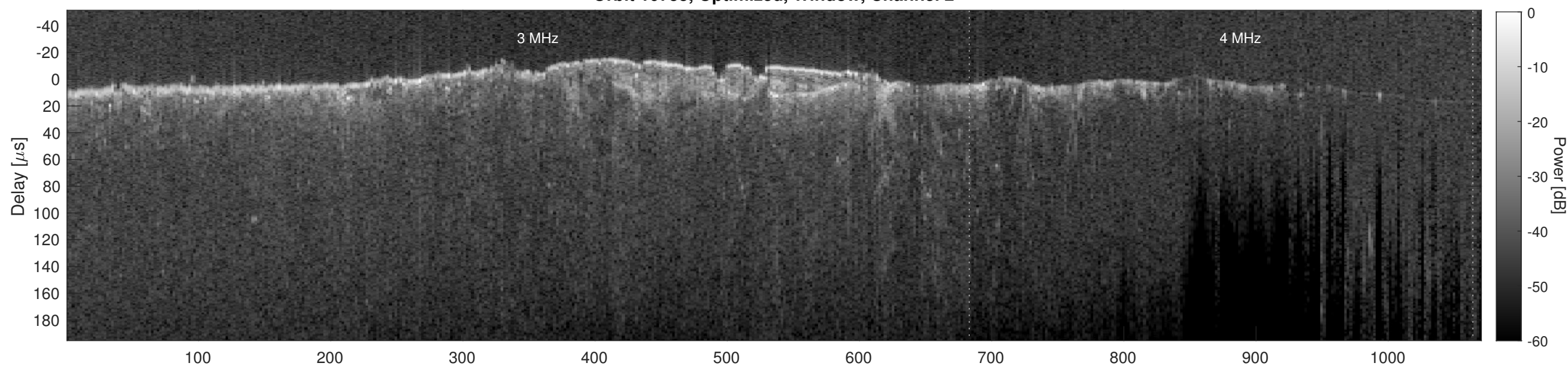
Orbit 10755, Cluttergram
