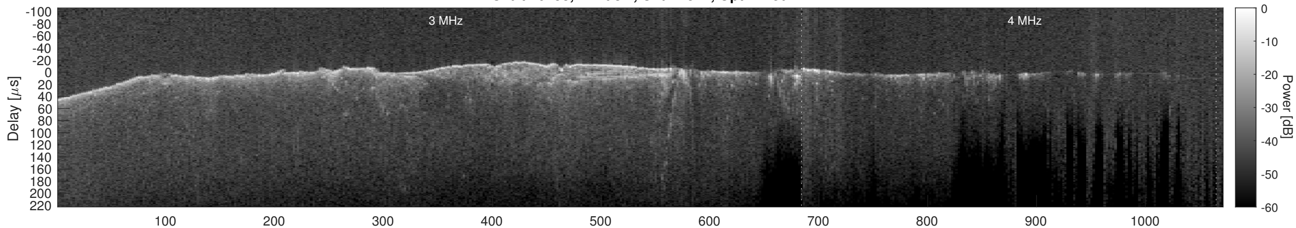
Orbit 10758, Cluttergram
