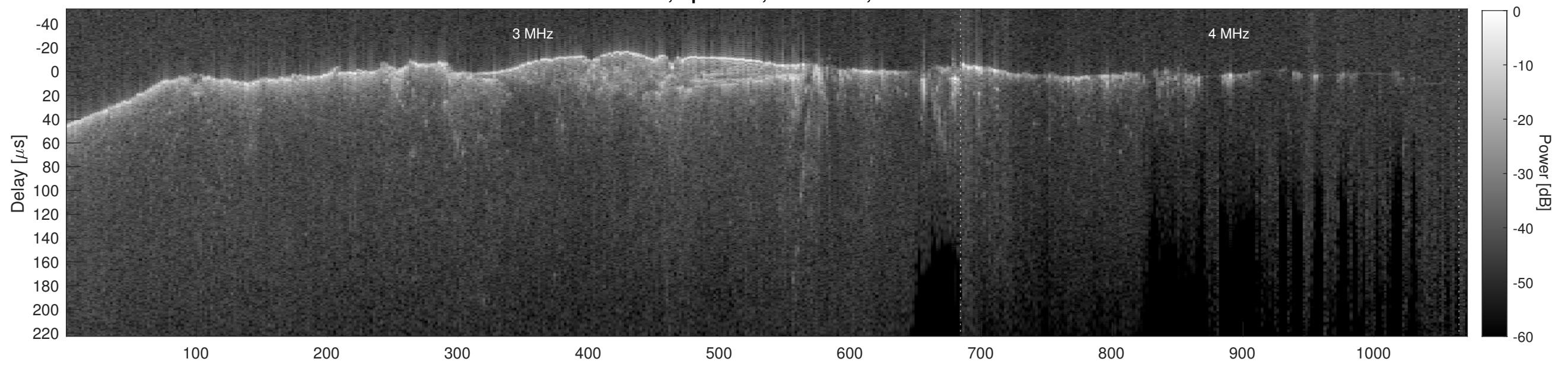
Orbit 10758, Cluttergram
