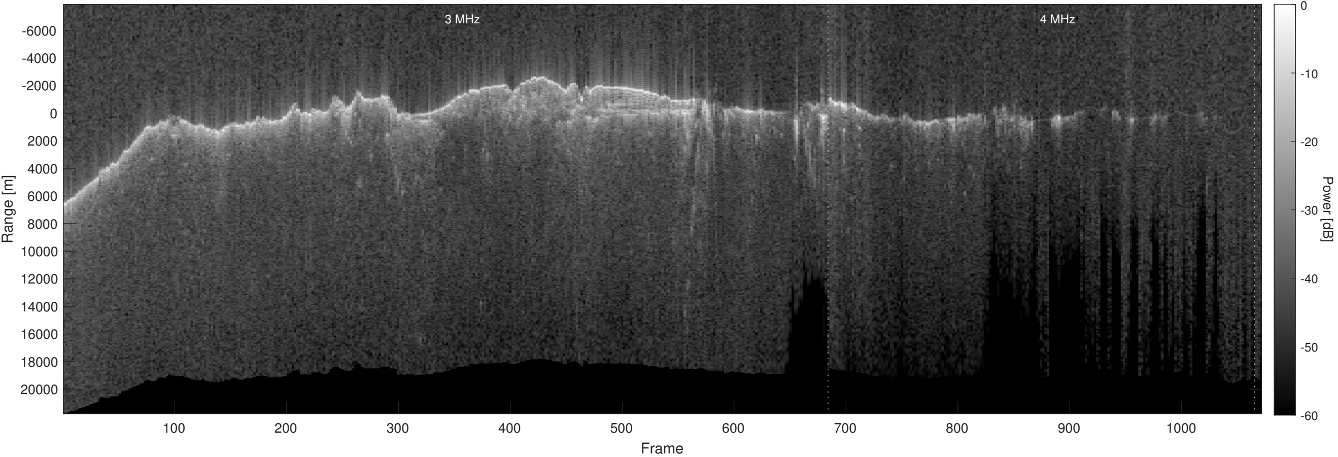
Orbit 10758, Optimized, No Window, Depth-Corrected, Channel 2
