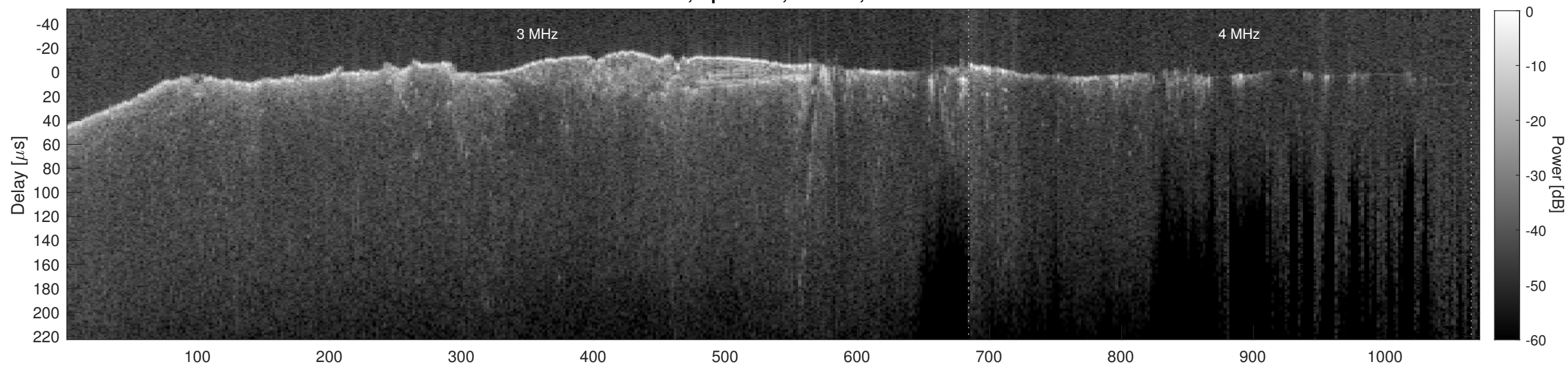
Orbit 10758, Cluttergram
