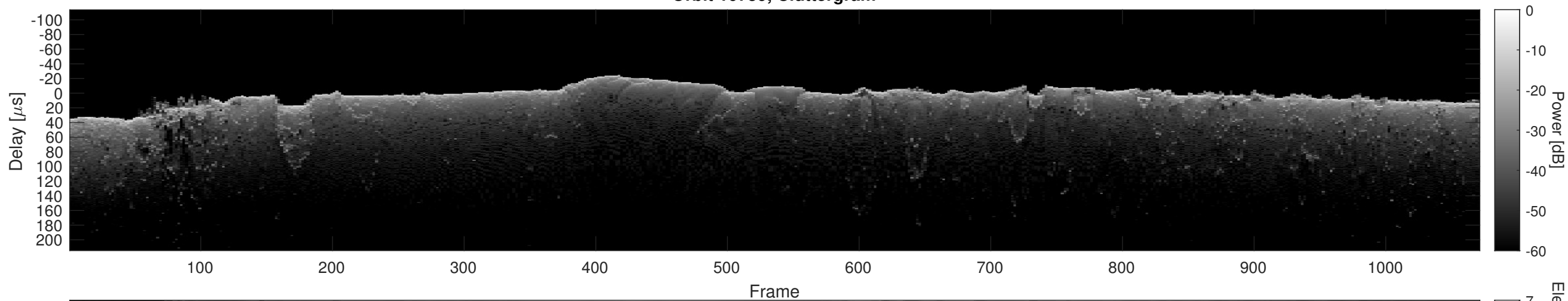
Orbit 10759, Cluttergram
