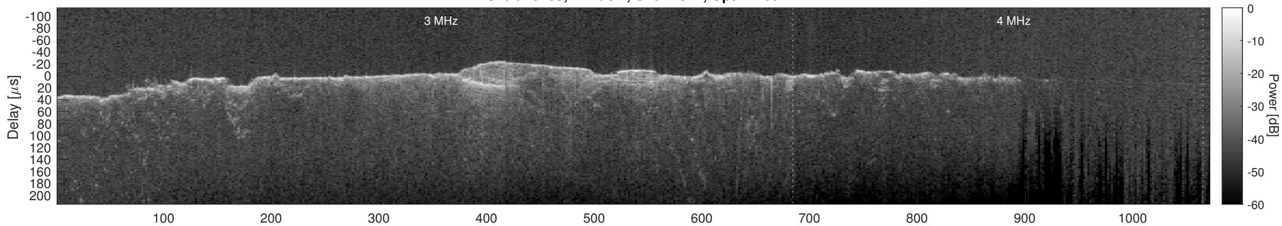
Orbit 10759, Cluttergram
