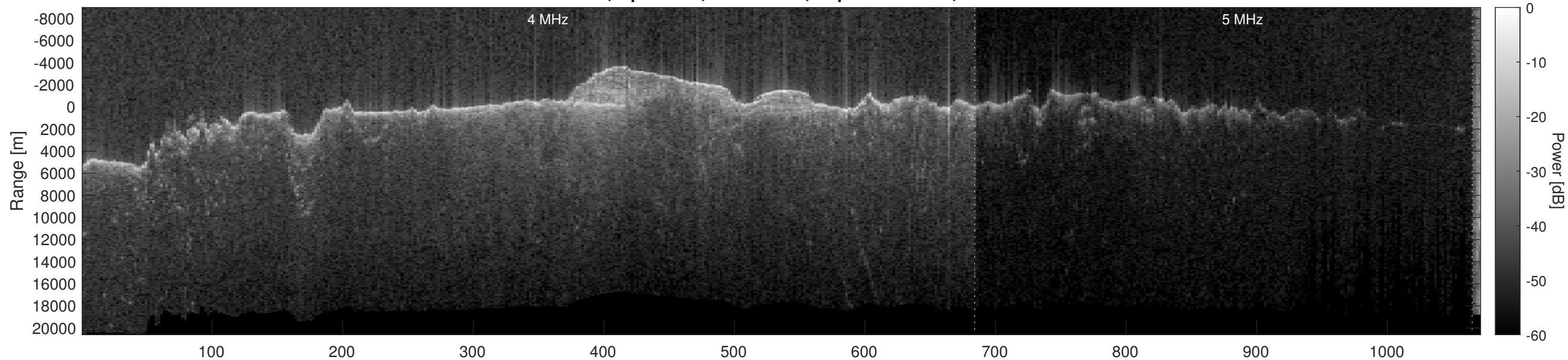
Orbit 10759, Optimized, No Window, Depth-Corrected, Channel 2
