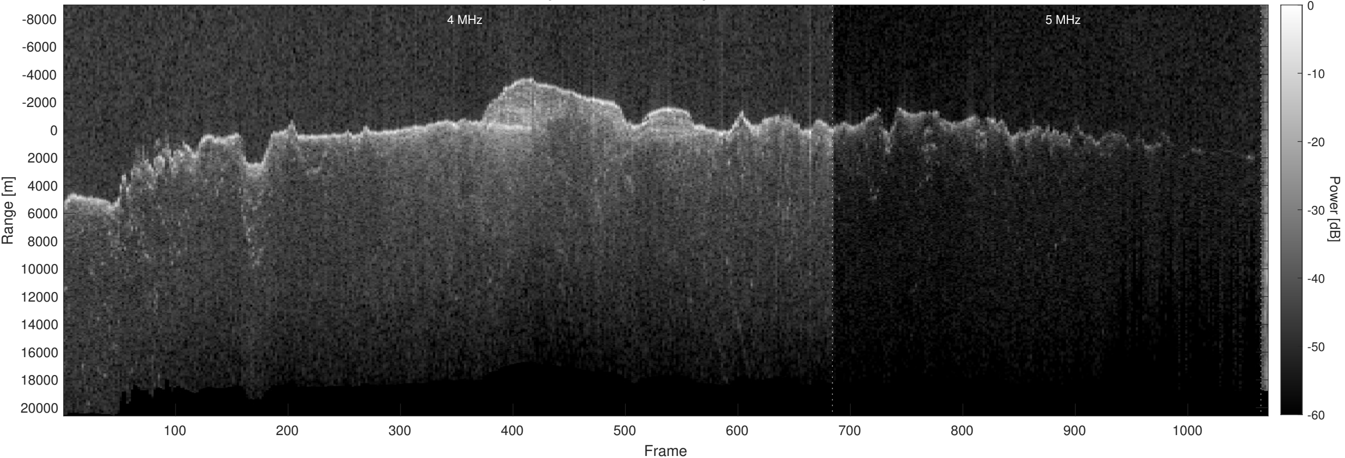
Orbit 10759, Optimized, Window, Depth-Corrected, Channel 2
