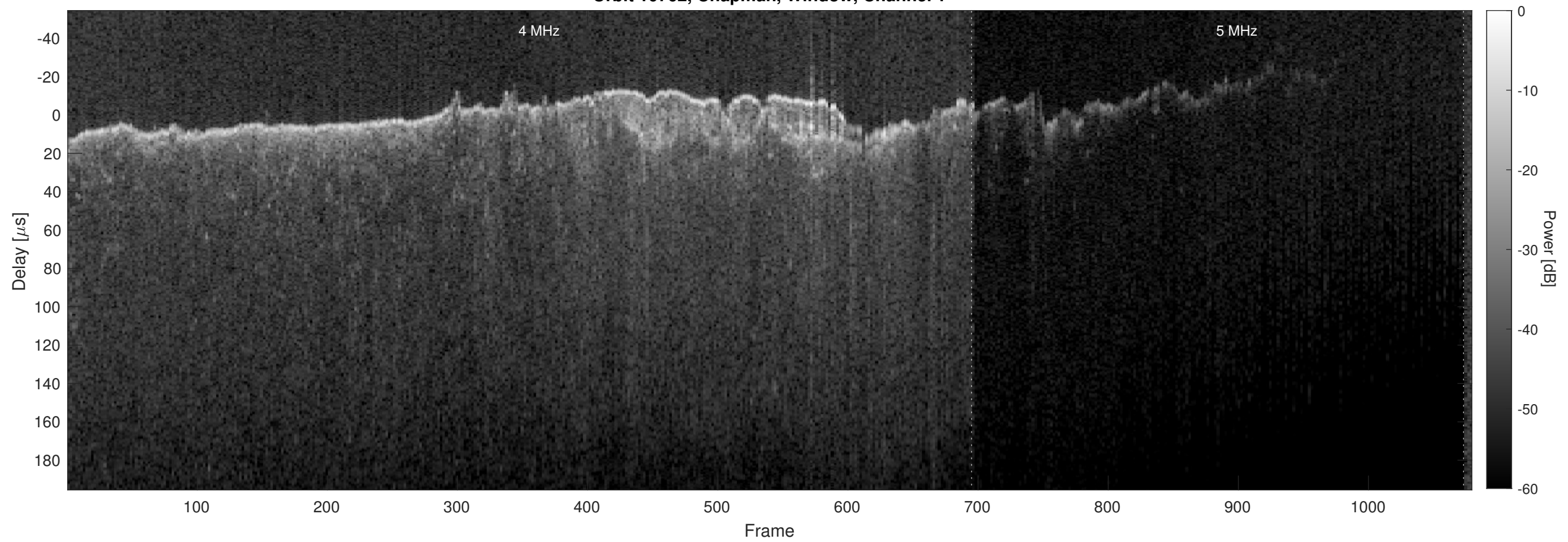
Orbit 10762, Chapman, Window, Channel 2
