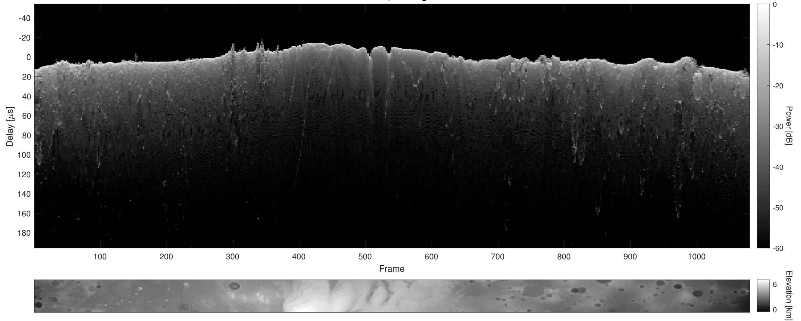
Orbit 10762, Cluttergram
