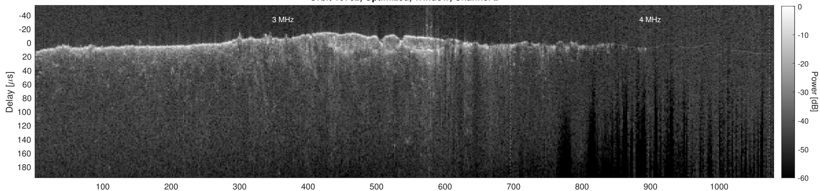
Orbit 10762, Cluttergram
