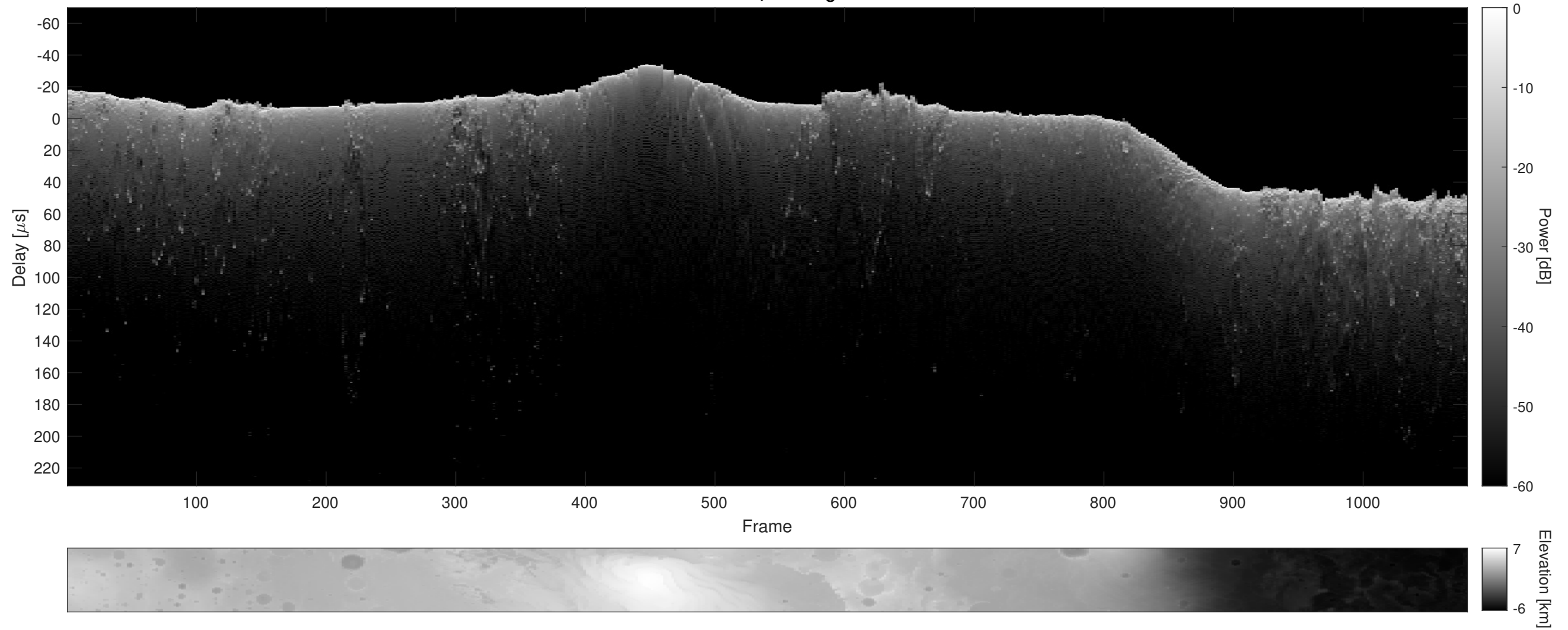
Orbit 10763, Cluttergram
