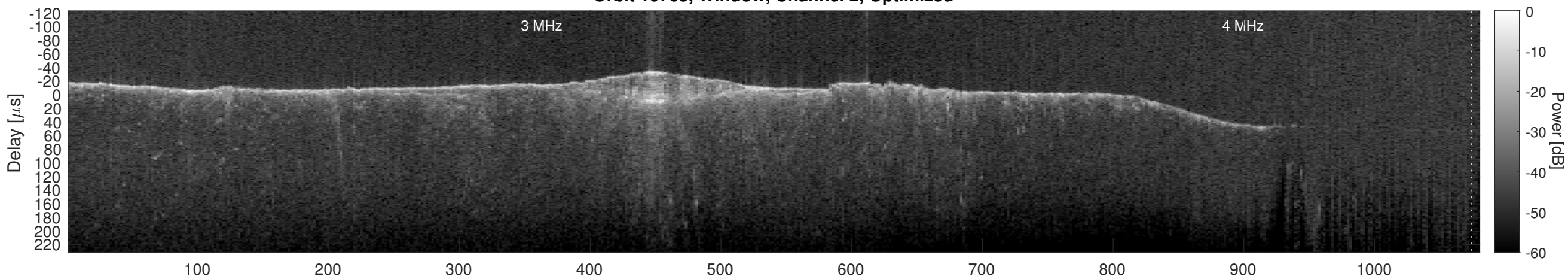
Orbit 10763, Cluttergram
