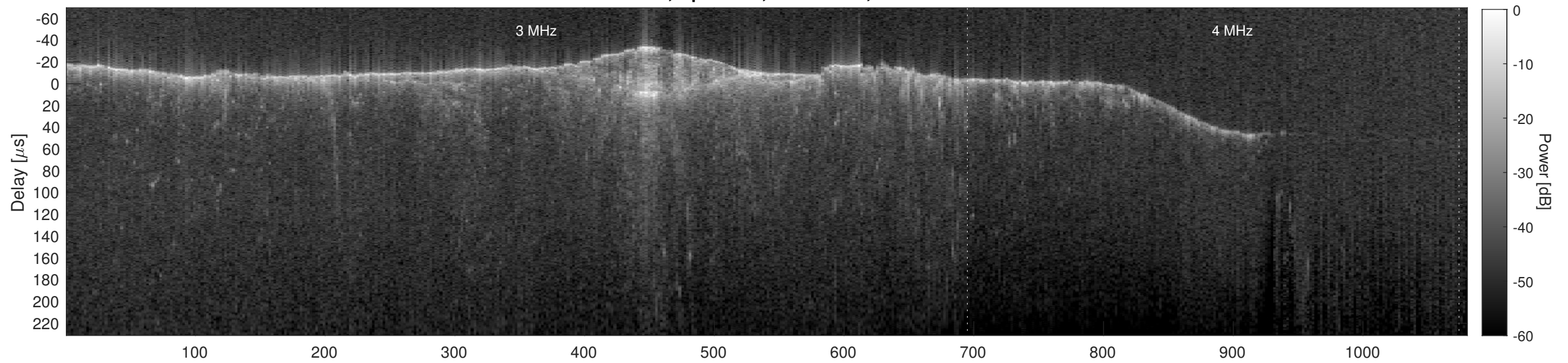
Orbit 10763, Cluttergram
