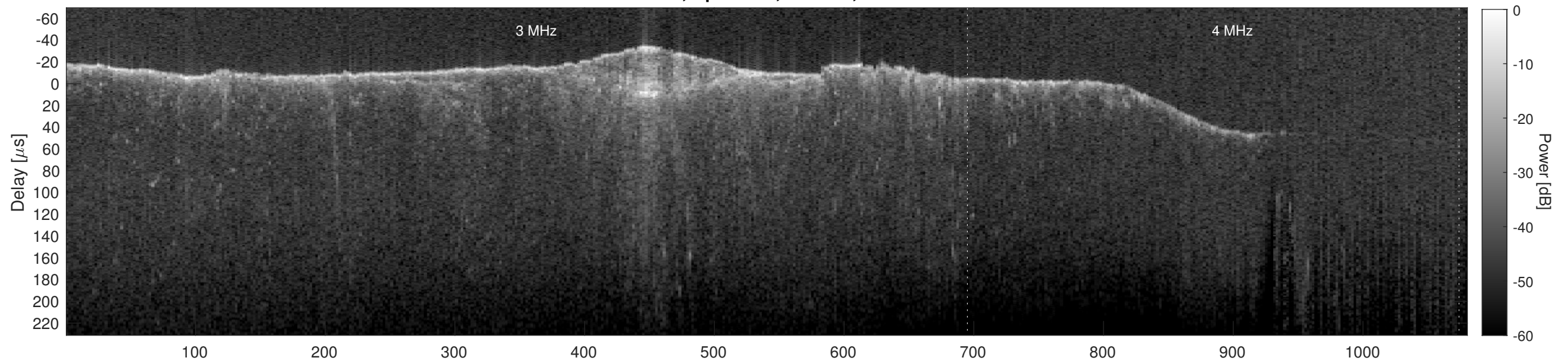
Orbit 10763, Cluttergram
