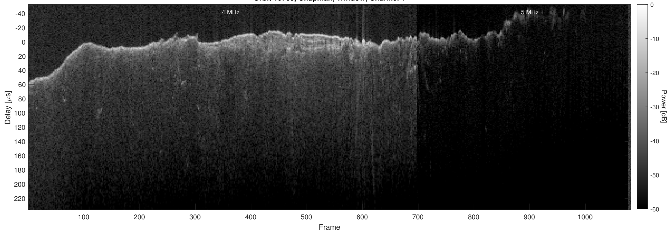
Orbit 10765, Chapman, Window, Channel 2
