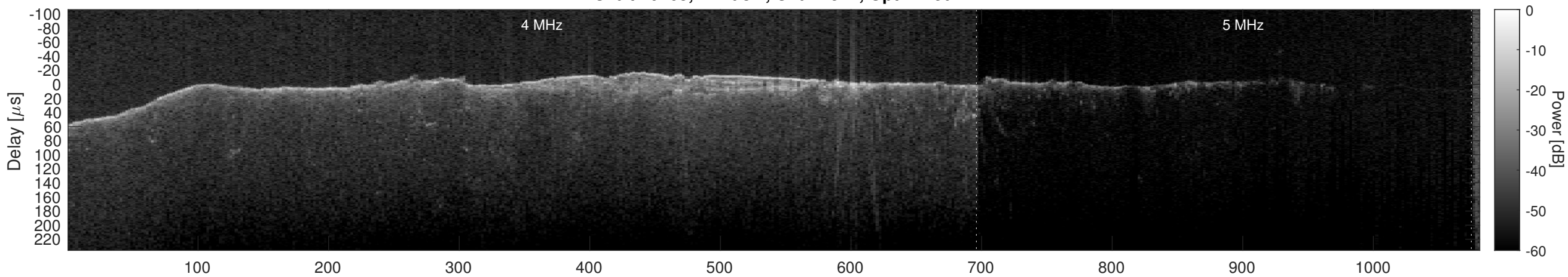
Orbit 10765, Cluttergram
