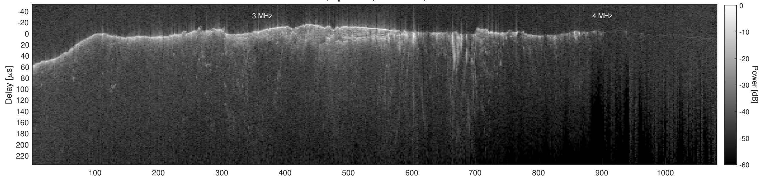
Orbit 10765, Cluttergram
