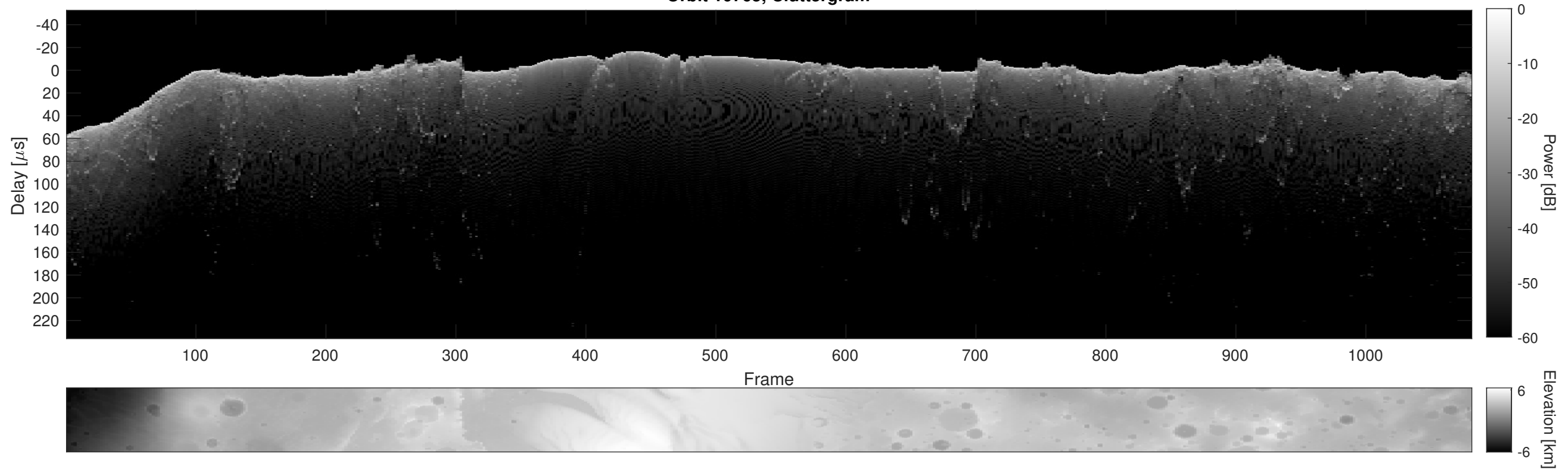
Orbit 10765, Cluttergram
