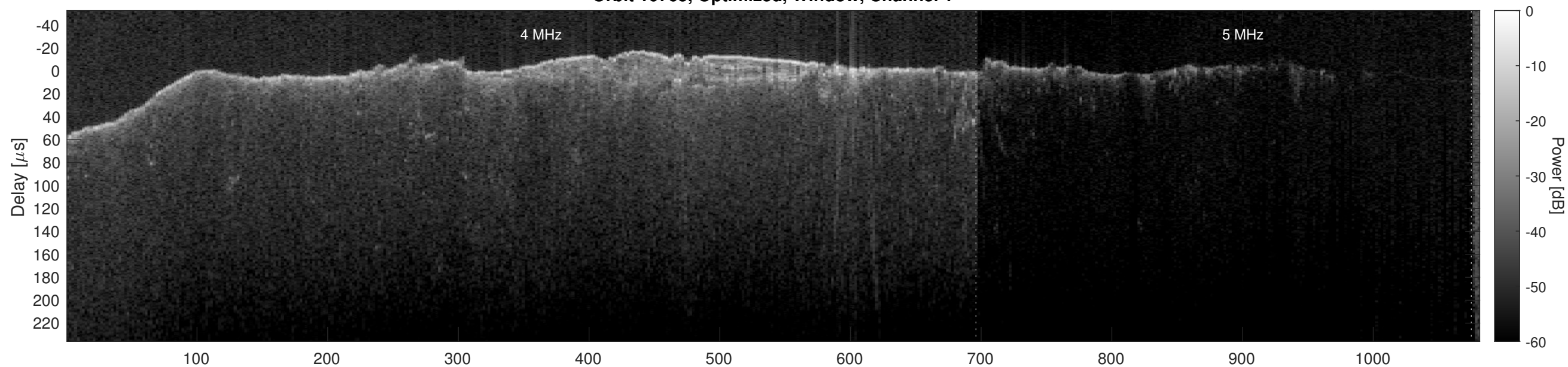
Orbit 10765, Optimized, Window, Channel 2
