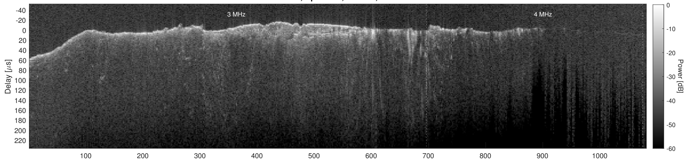
Orbit 10765, Cluttergram
