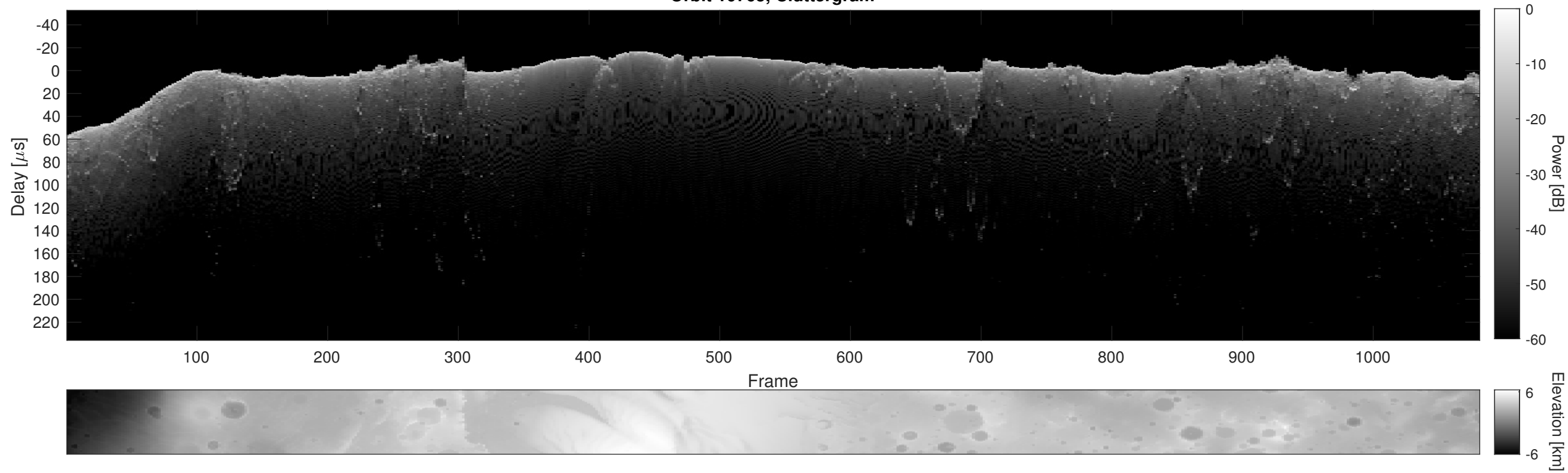
Orbit 10765, Cluttergram
