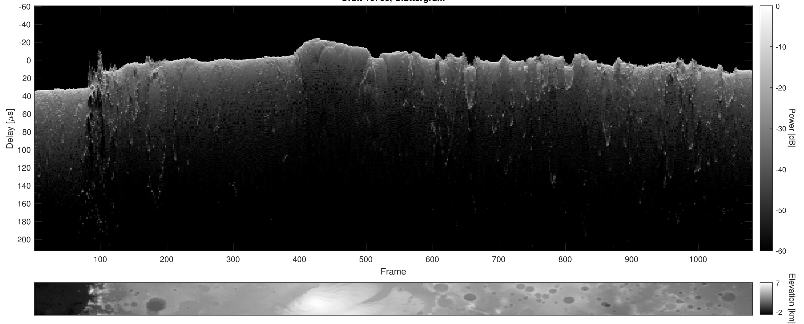
Orbit 10766, Cluttergram
