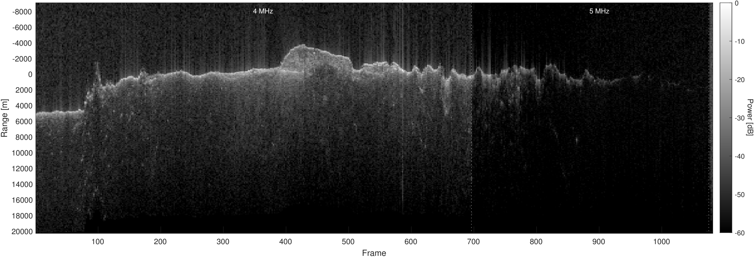
Orbit 10766, Optimized, No Window, Depth-Corrected, Channel 2
