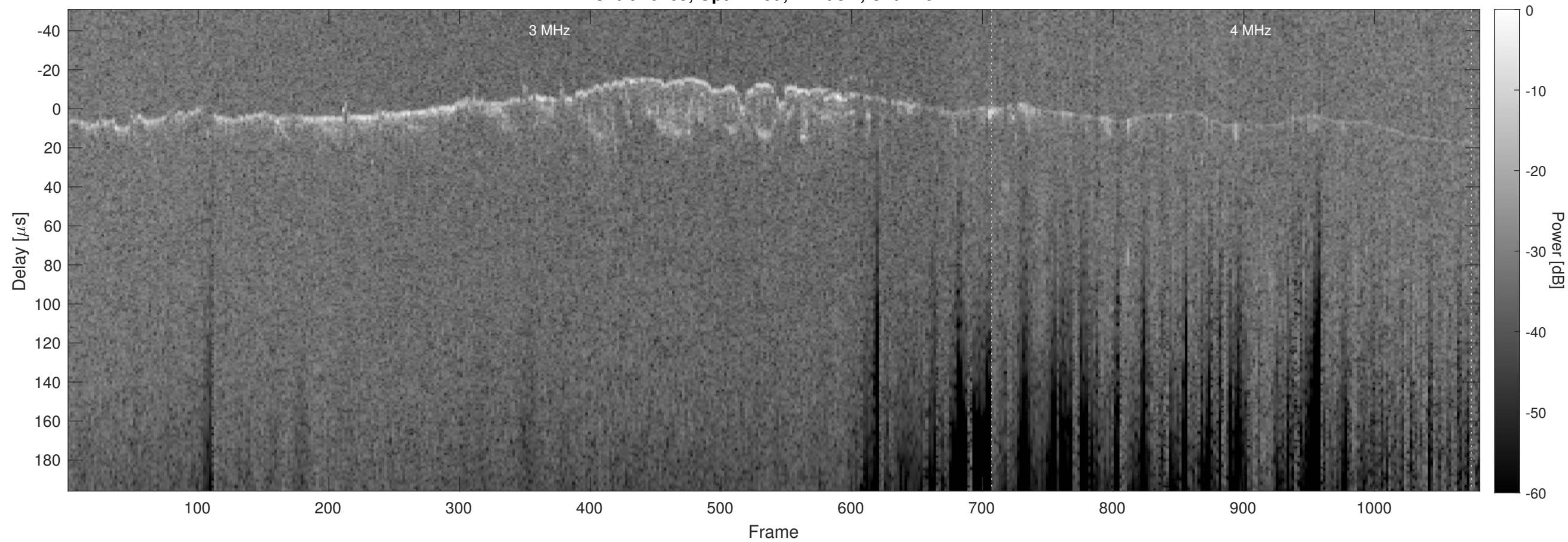
Orbit 10769, Optimized, Window, Channel 2
