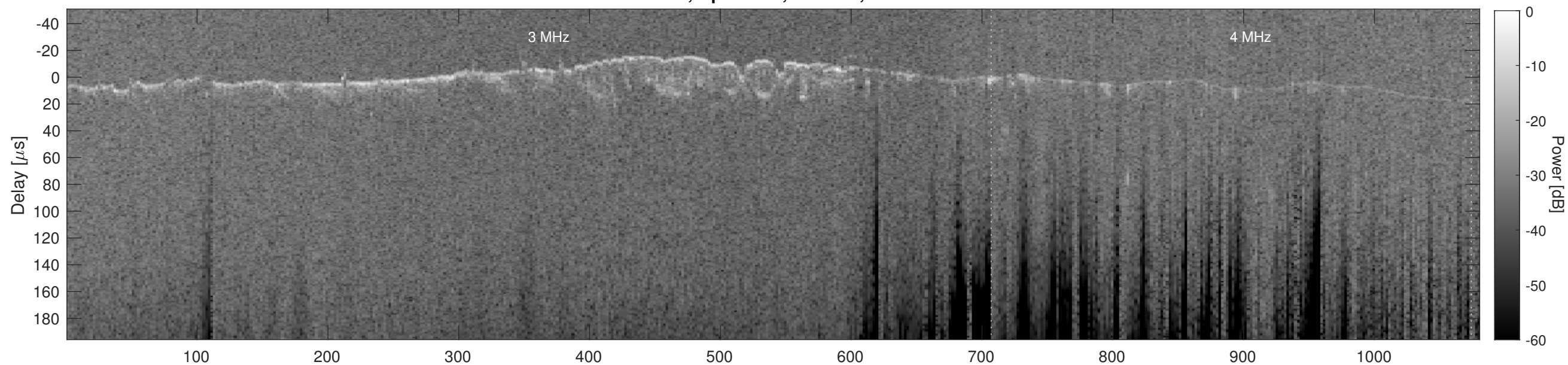
Orbit 10769, Cluttergram
