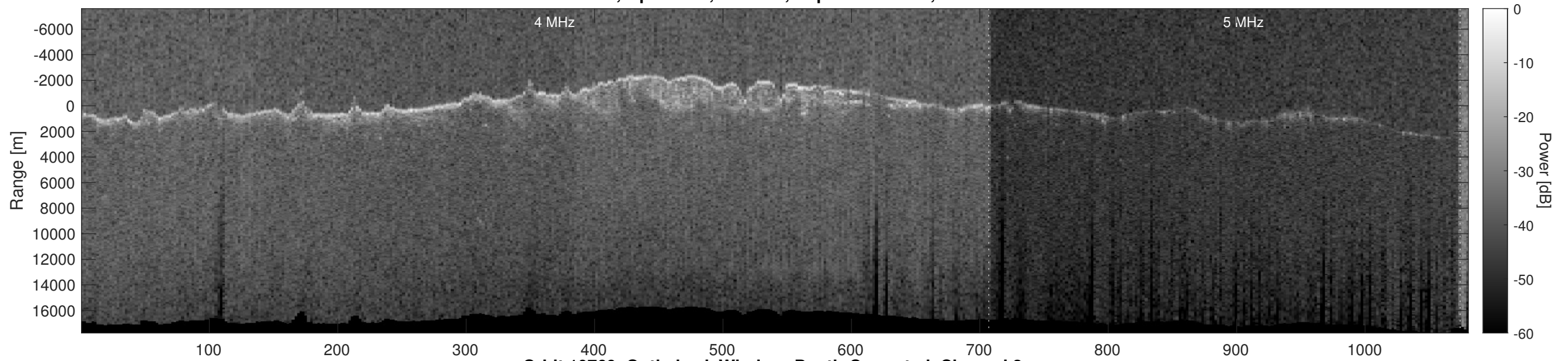
Orbit 10769, Optimized, Window, Depth-Corrected, Channel 2
