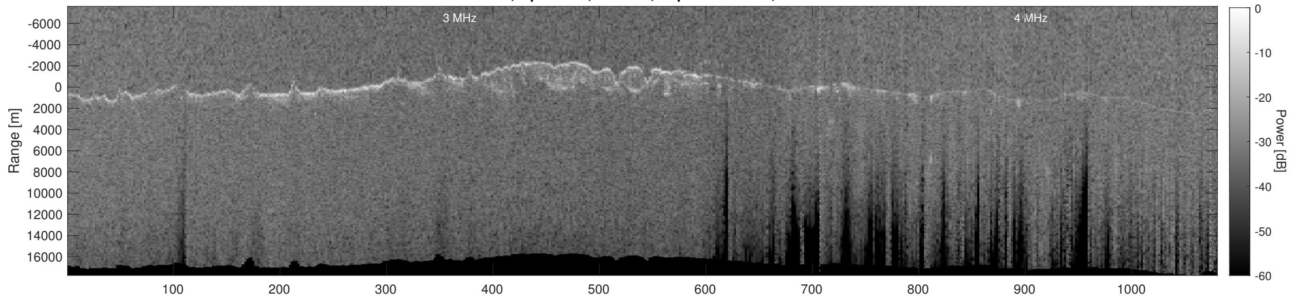
Orbit 10769, Depth-Corrected Cluttergram
