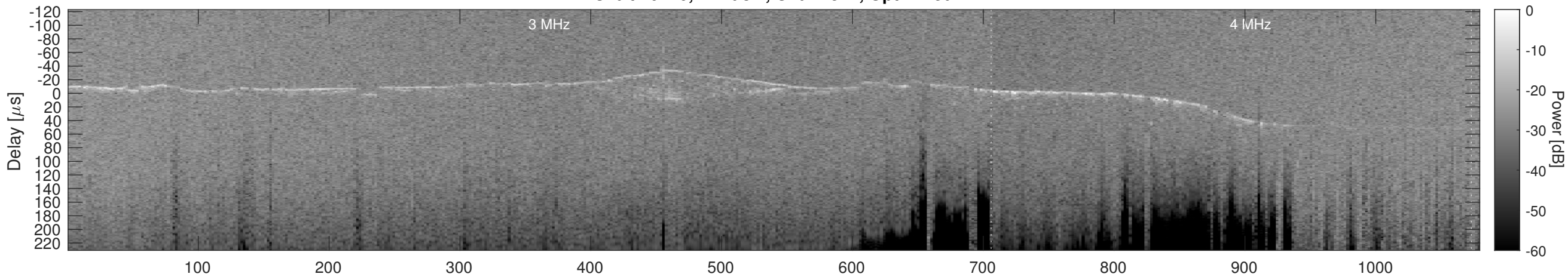
Orbit 10770, Cluttergram
