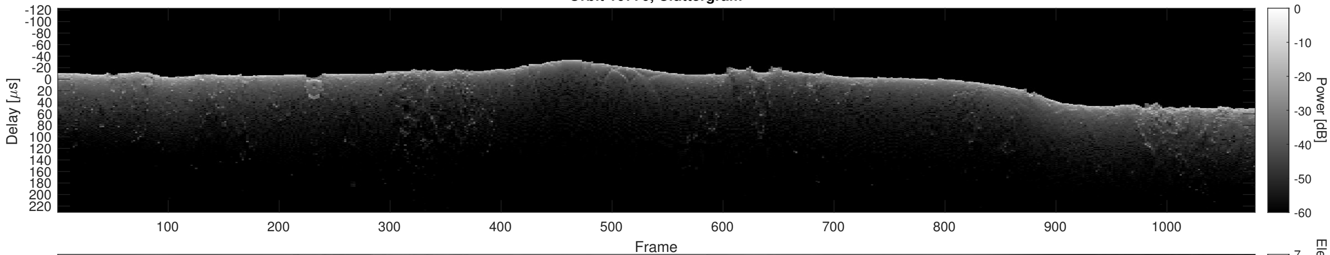
Orbit 10770, Cluttergram
