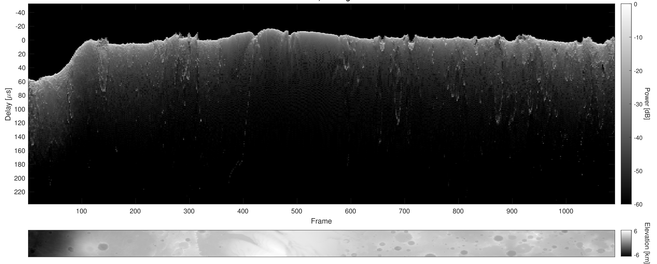
Orbit 10772, Cluttergram
