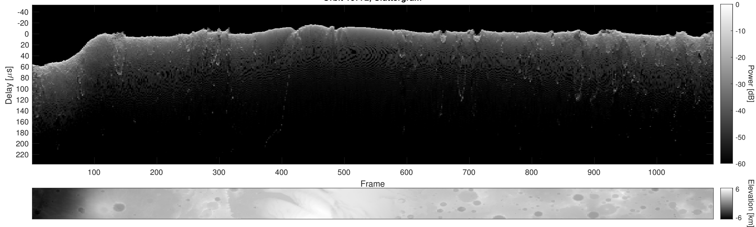
Orbit 10772, Cluttergram
