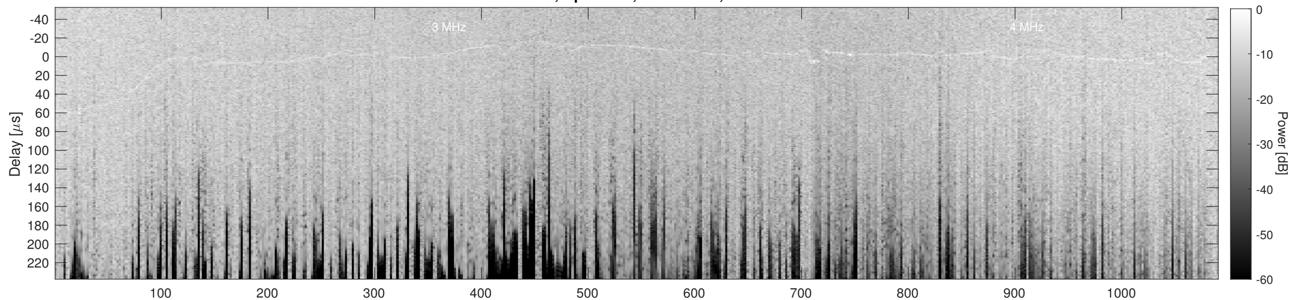
Orbit 10772, Cluttergram
