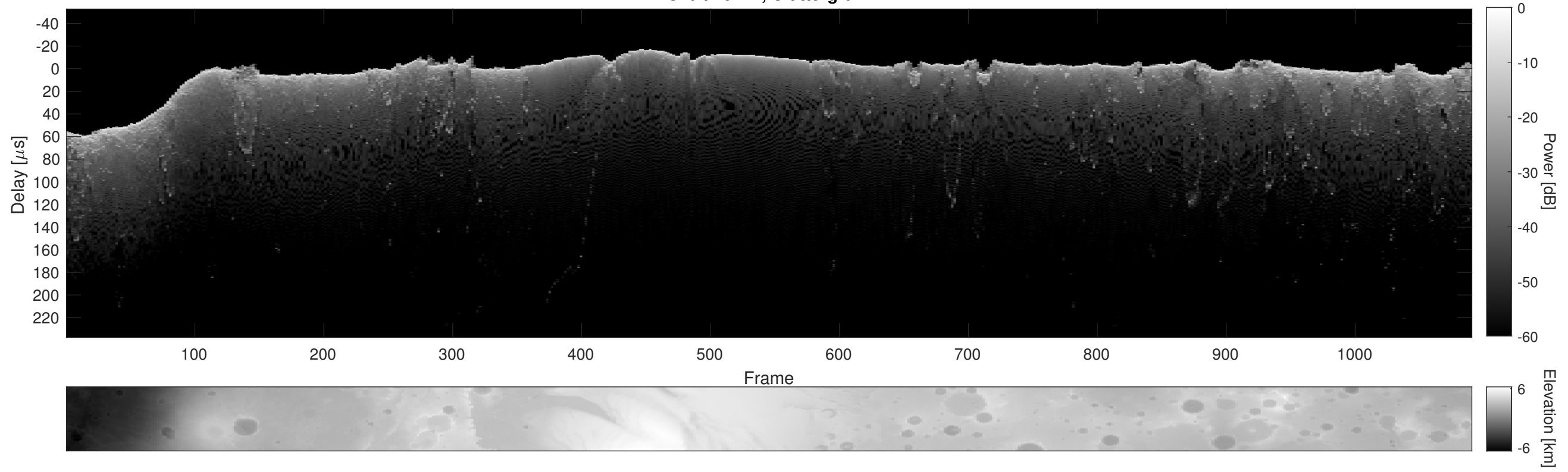
Orbit 10772, Cluttergram
