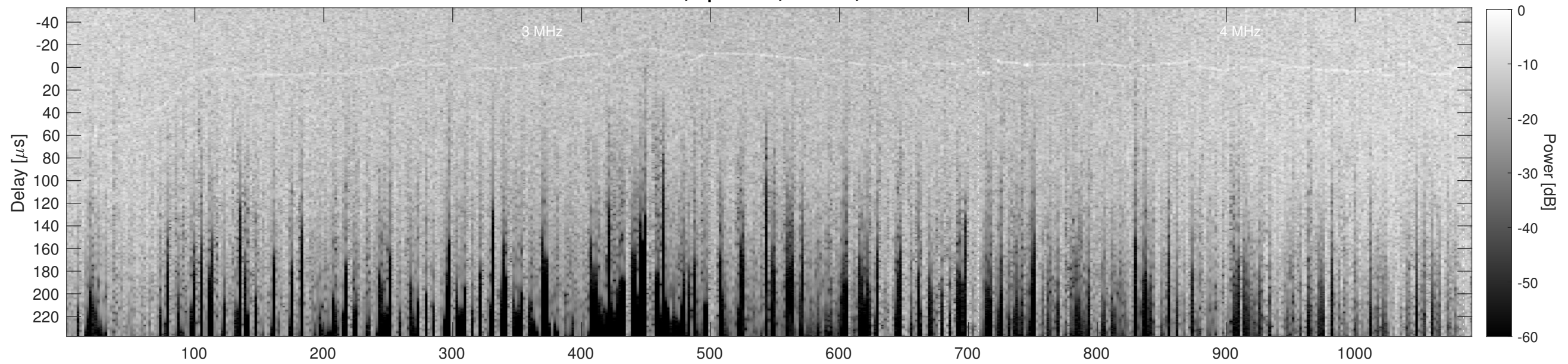
Orbit 10772, Cluttergram
