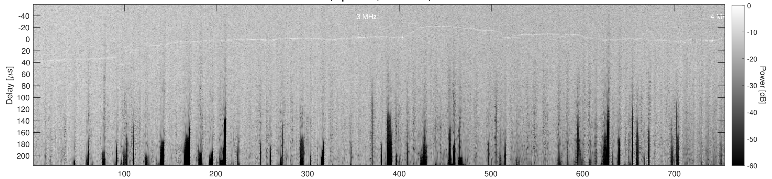
Orbit 10773, Cluttergram
