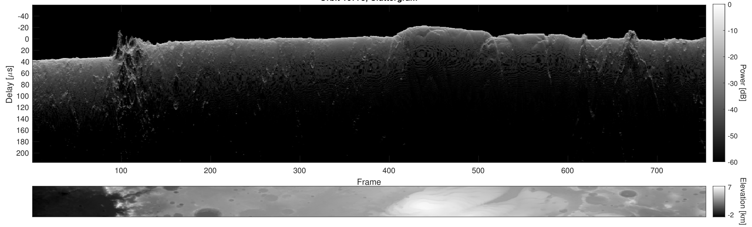
Orbit 10773, Cluttergram
