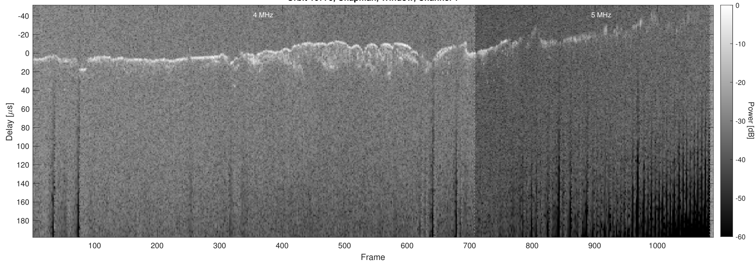
Orbit 10776, Chapman, Window, Channel 2
