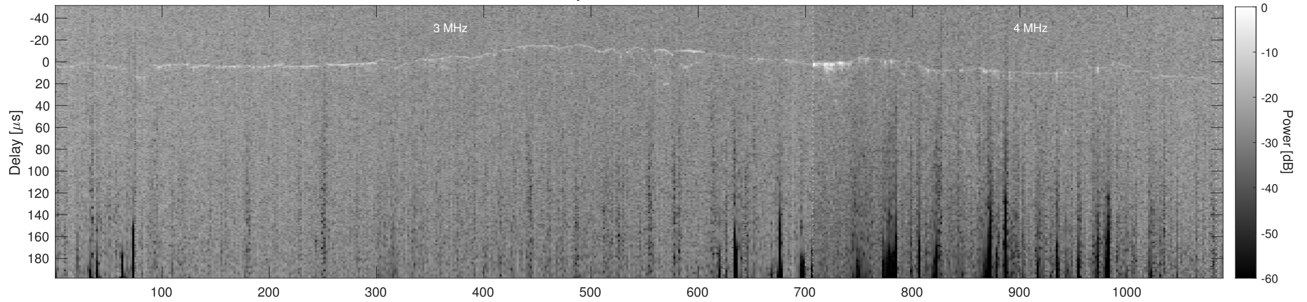
Orbit 10776, Cluttergram
