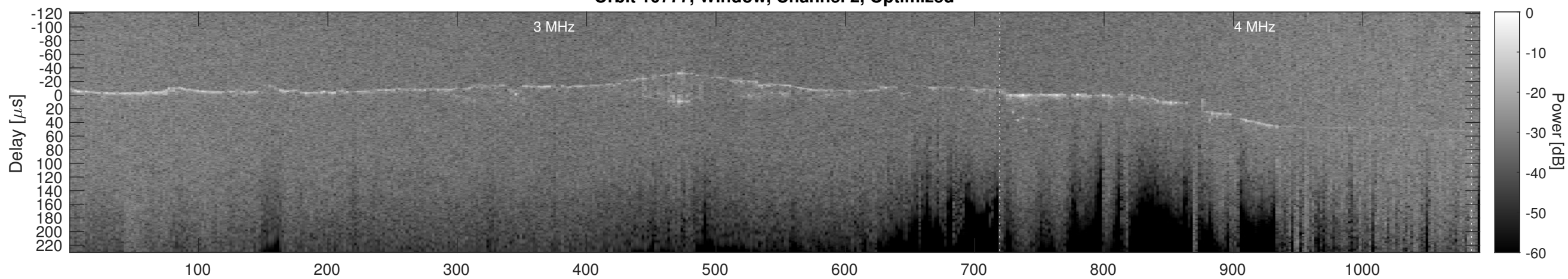
Orbit 10777, Cluttergram
