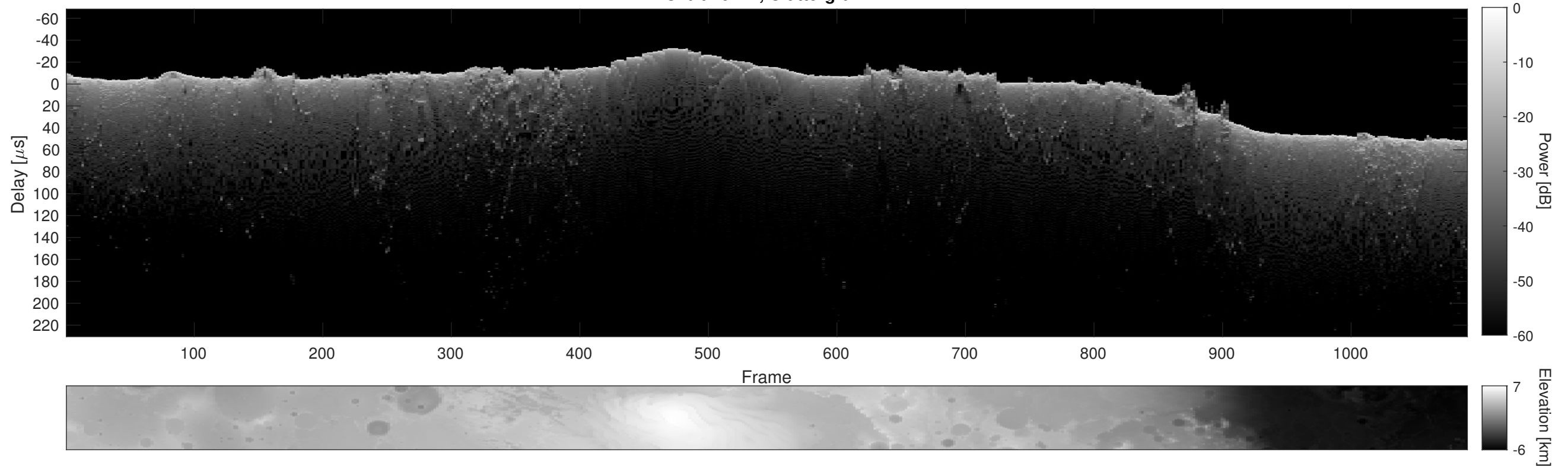
Orbit 10777, Cluttergram
