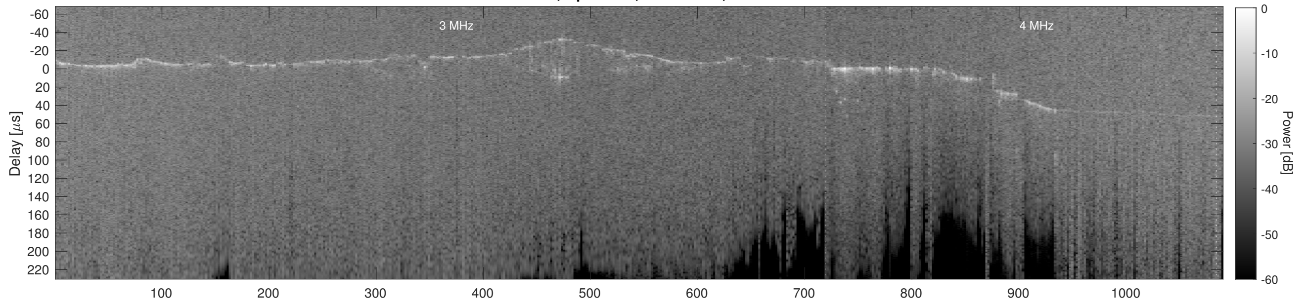
Orbit 10777, Cluttergram
