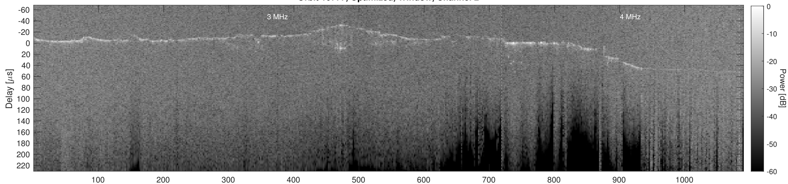
Orbit 10777, Cluttergram
