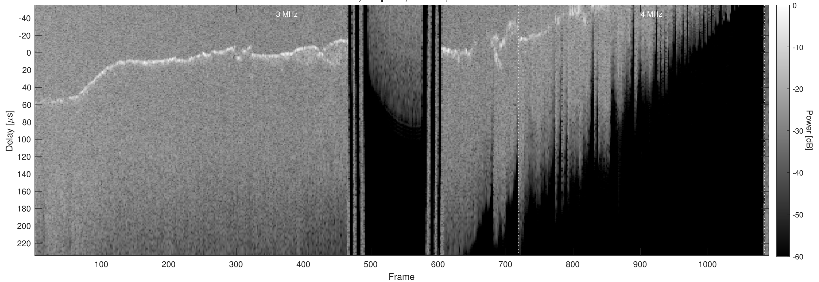
Orbit 10779, Chapman, Window, Channel 2
