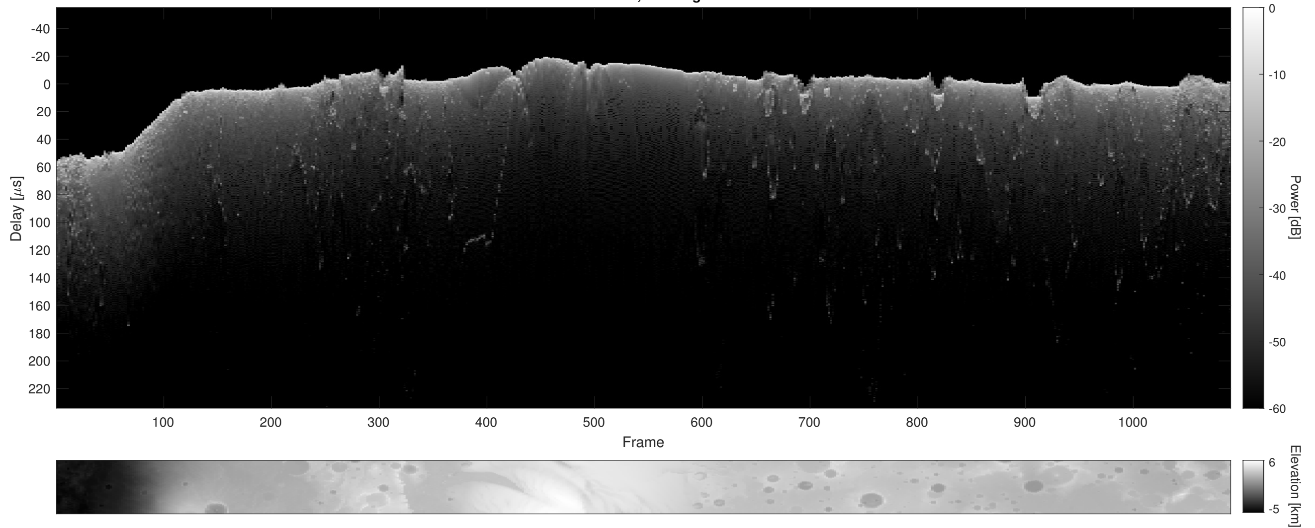
Orbit 10779, Cluttergram
