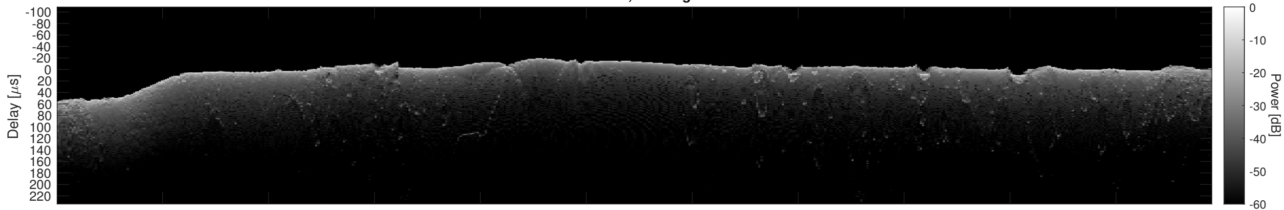
Orbit 10779, Cluttergram
