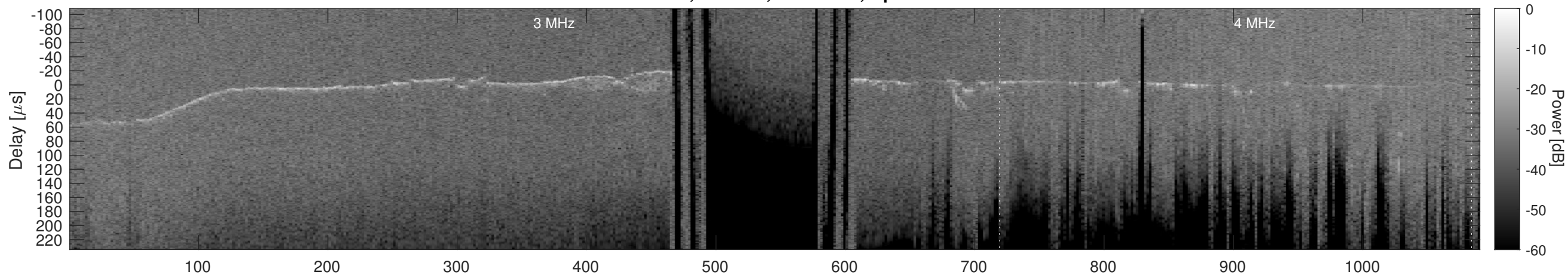
Orbit 10779, Cluttergram
