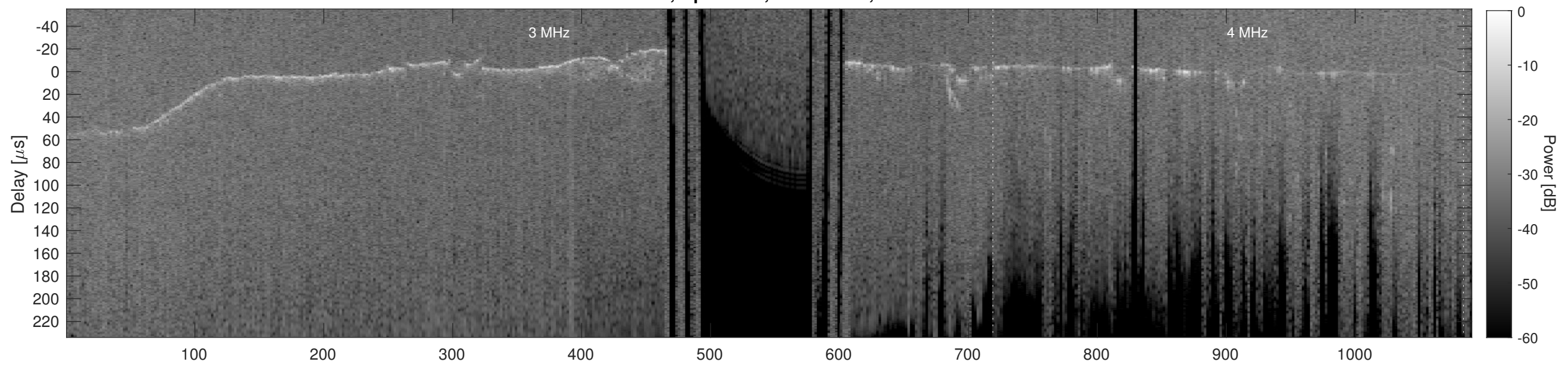
Orbit 10779, Cluttergram
