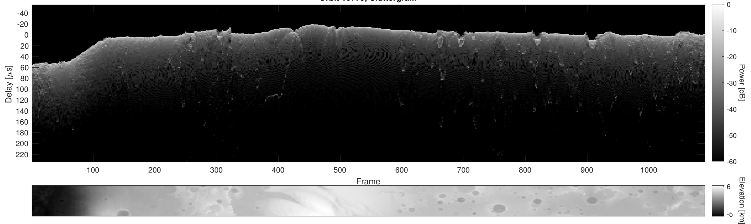
Orbit 10779, Cluttergram
