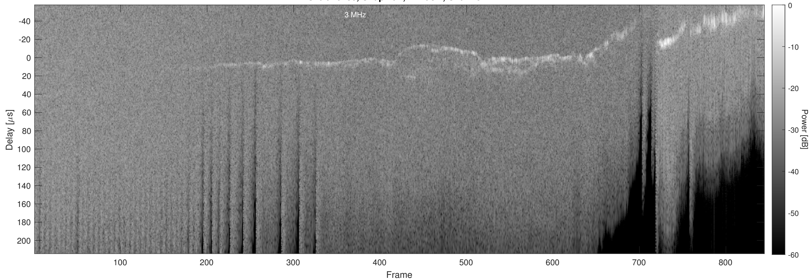
Orbit 10780, Chapman, Window, Channel 2
