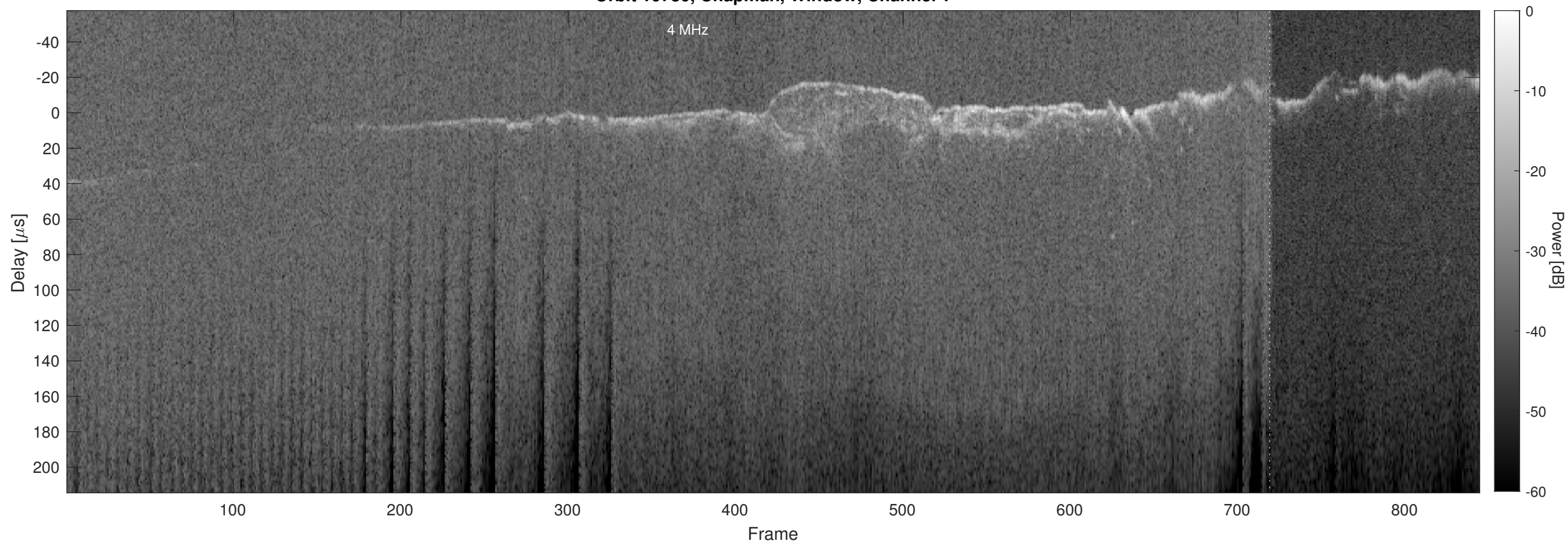
Orbit 10780, Chapman, Window, Channel 2
