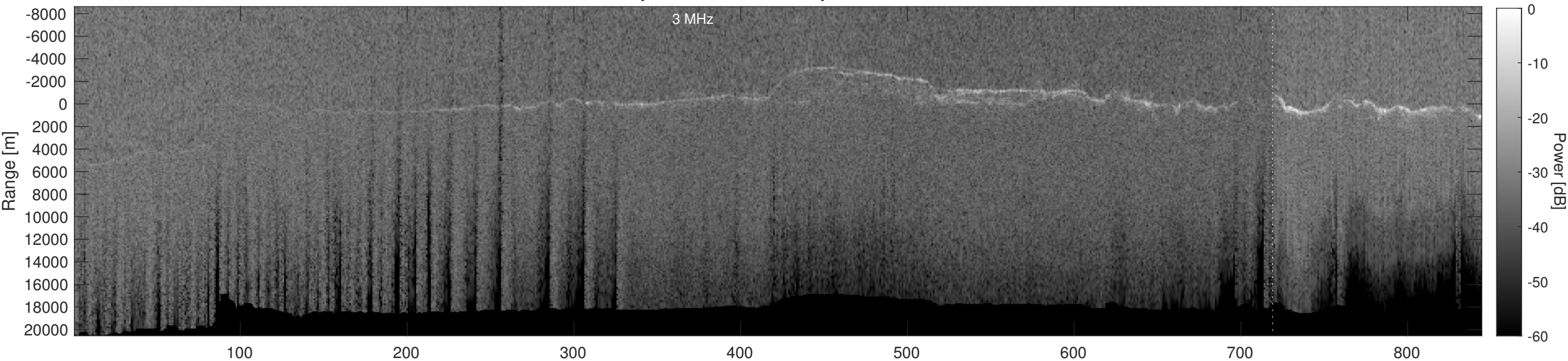
Orbit 10780, Depth-Corrected Cluttergram
