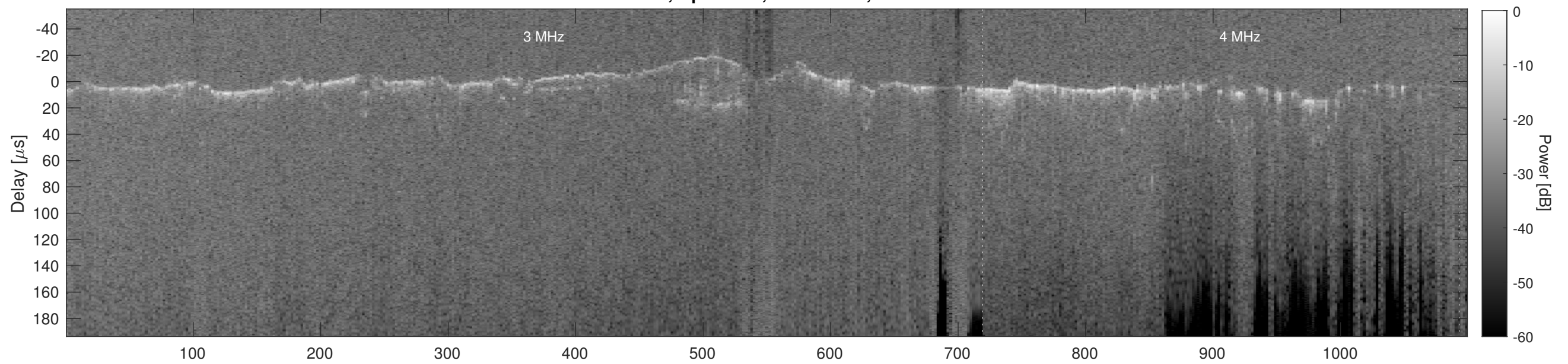
Orbit 10781, Cluttergram
