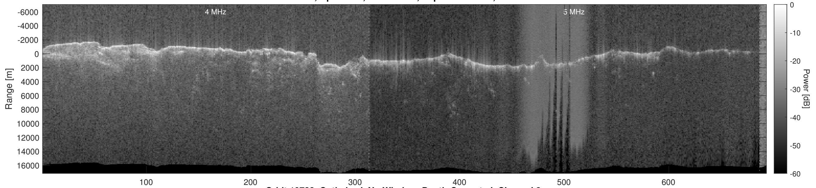
Orbit 10782, Optimized, No Window, Depth-Corrected, Channel 2
