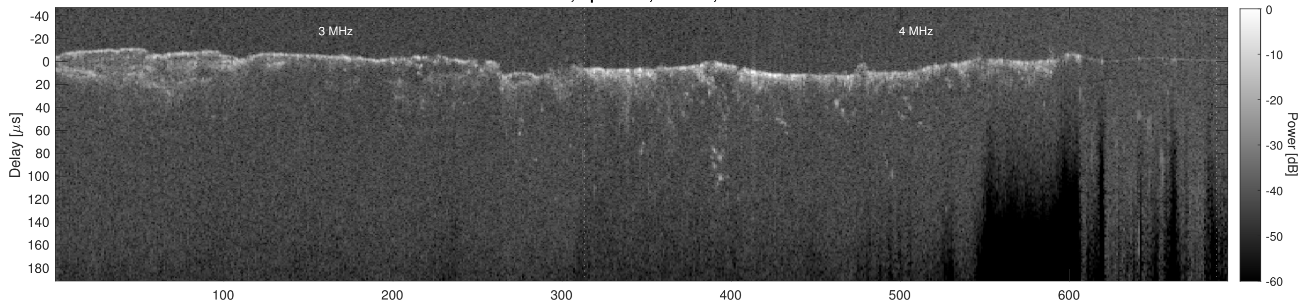
Orbit 10782, Cluttergram
