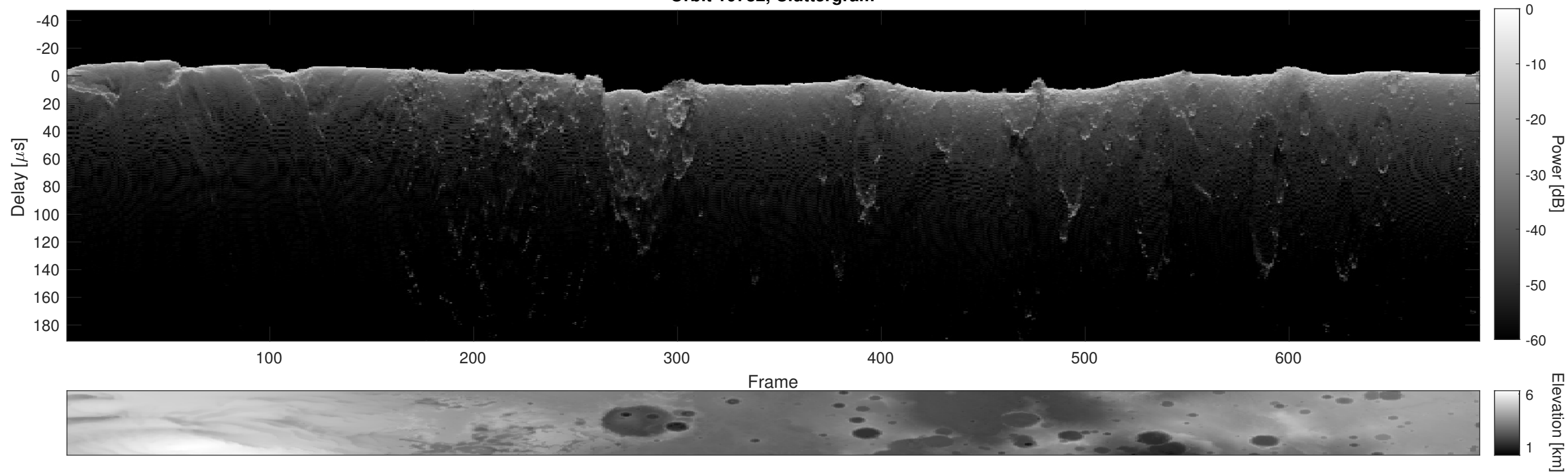
Orbit 10782, Cluttergram
